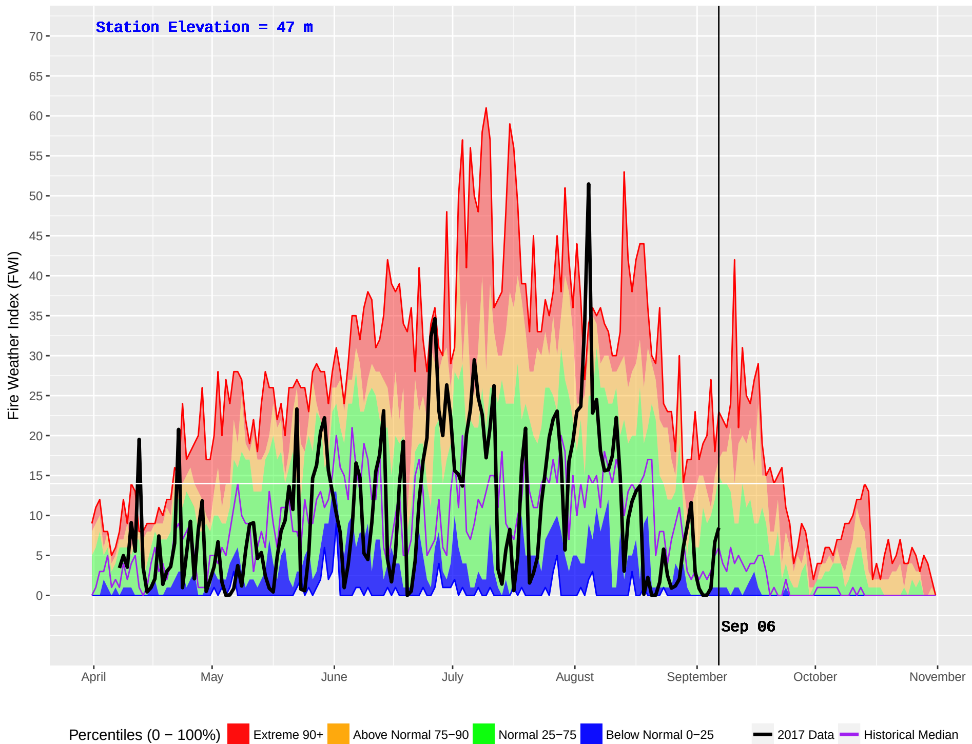
HAGENSBORG 2 (904) : Historical (2005–2016) and Current (2017) Noon Fire Weather Index (FWI)
