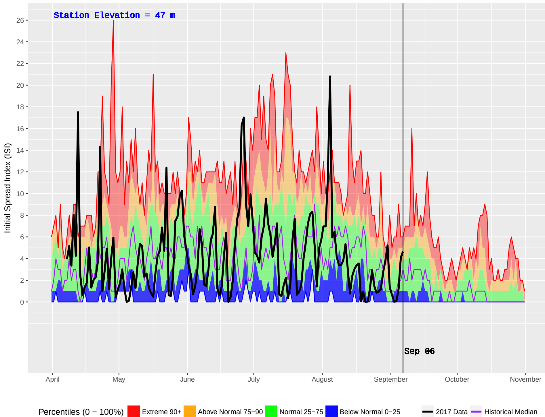
HAGENSBORG 2 (904) : Historical (2005–2016) and Current (2017) Noon Initial Spread Index (ISI)
