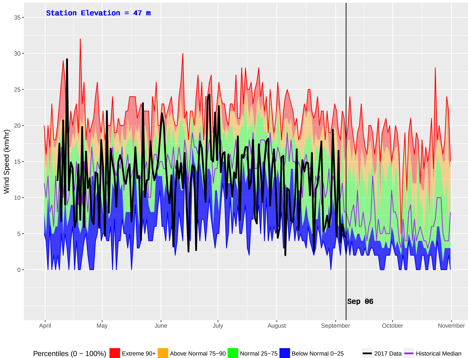
HAGENSBORG 2 (904) : Historical (2005–2016) and Current (2017) Noon Wind Speed
