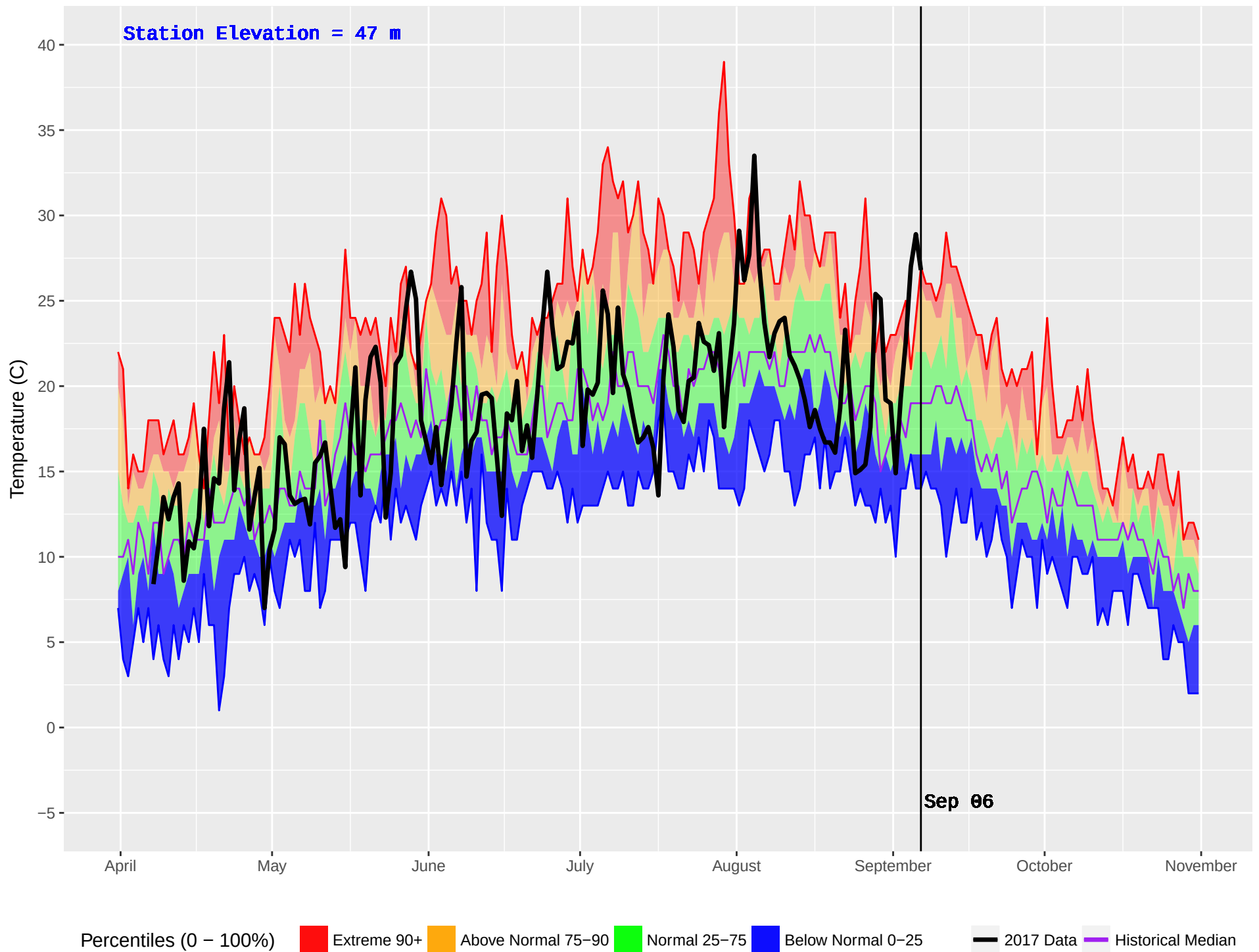
HAGENSBORG 2 (904) : Historical (2005–2016) and Current (2017) Noon Temperature
